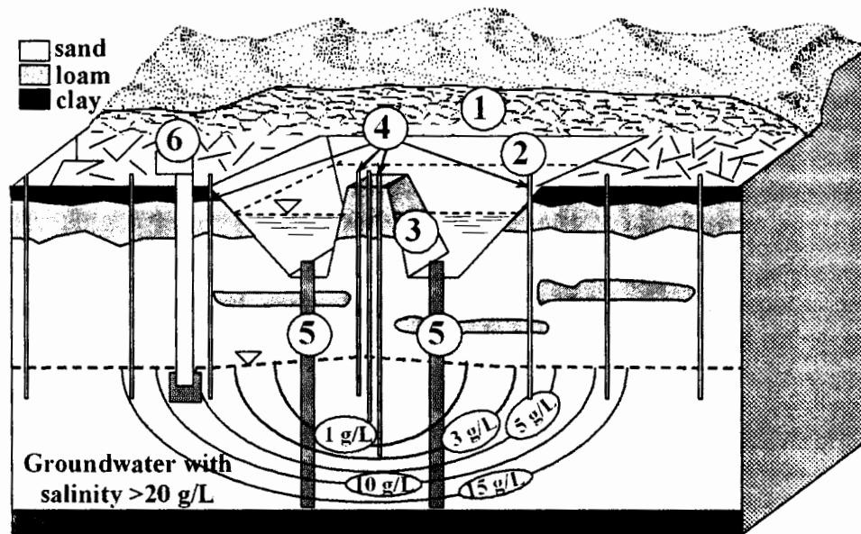
Figure 1. Experimental system for the ALFGW formation at the takyr Karrykul: 1- takyr watershed, 2- infiltration pond, 3- observation island, 4- observation boreholes, 5- recharging wells, 6- exploitation well.
