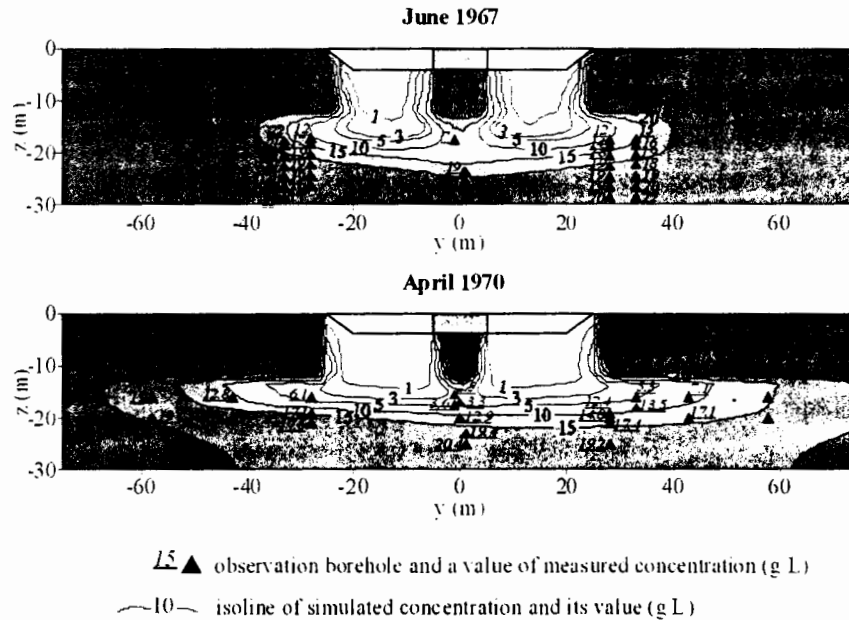
Figure 4. Measured and simulated spatial distribution of concentrations through a vertical cross-section at x=0 .
