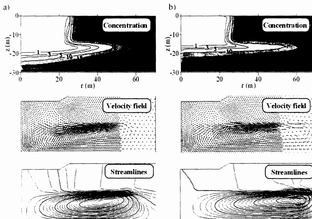
Figure 5. Simulated distributions of concentration (g/L), velocity field and streamlines: after 5 years of 5000 m 3 ALFGW replenishment per year; after additional 5 years without the ALFGW replenishment.
