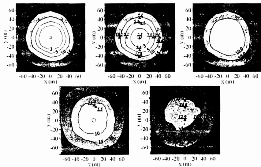
Figure 2. Measured and simulated areal distribution of concentrations at different depths in June 1967.
